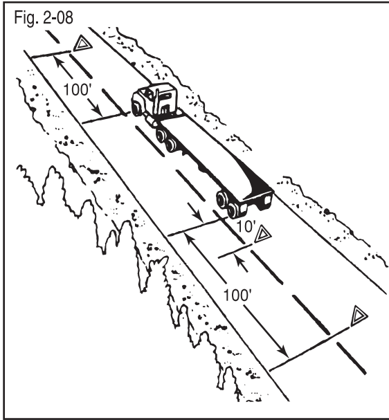
Warning Device Placement: Two-lane (traffic in both directions) or undivided highway
