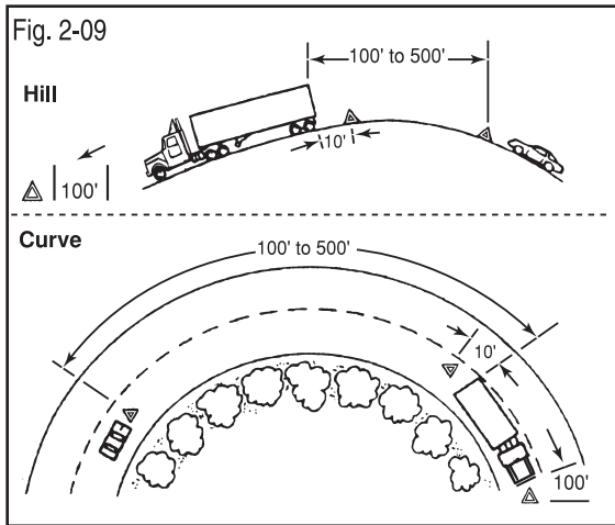
Warning Device Placement: Obstructed View
