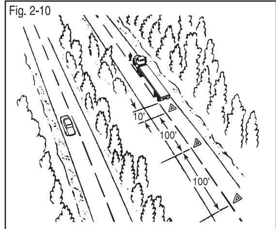
Warning Device Placement: One way or Divided Highway
