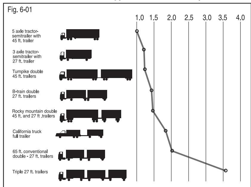
Influence of Combination Type on Rearward Amplification
